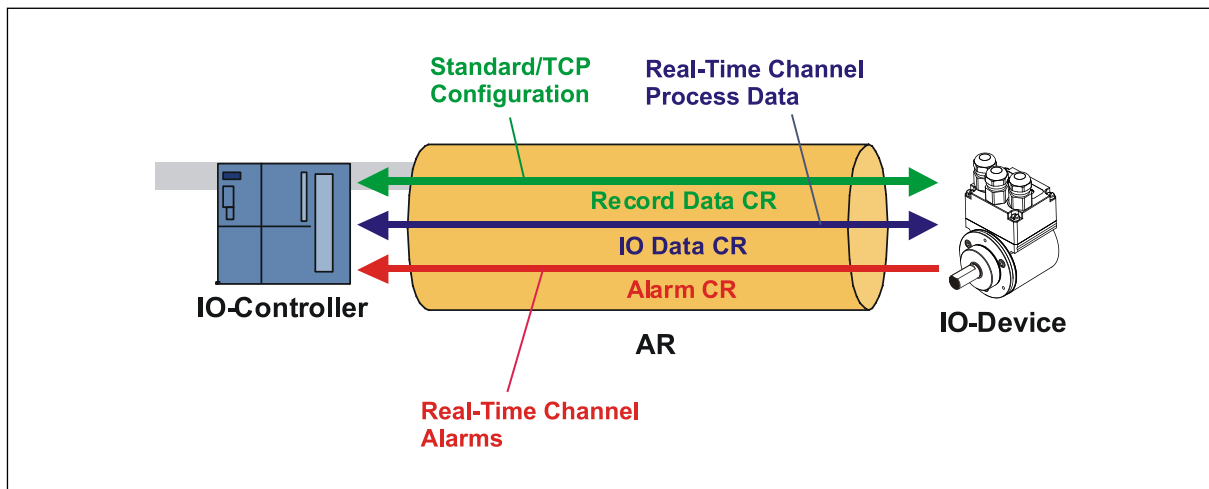
Figure 3: Device communication
